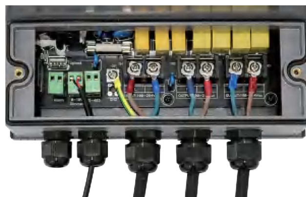
0-10V Signal
